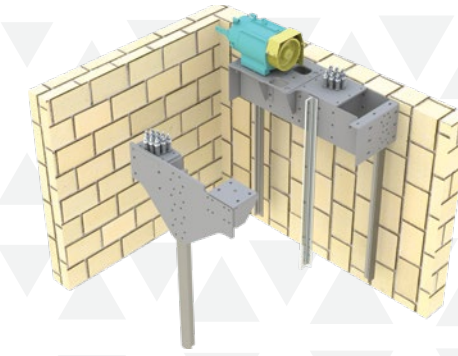
MC 03 MRL Duvara Bağlı Makine Şasesi MRL Wall Mounted Machine Chassis
