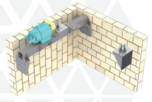
MC 04 MRL Raya Bağlı Makine Şasesi MRL Rail Mounted Machine Chassis
